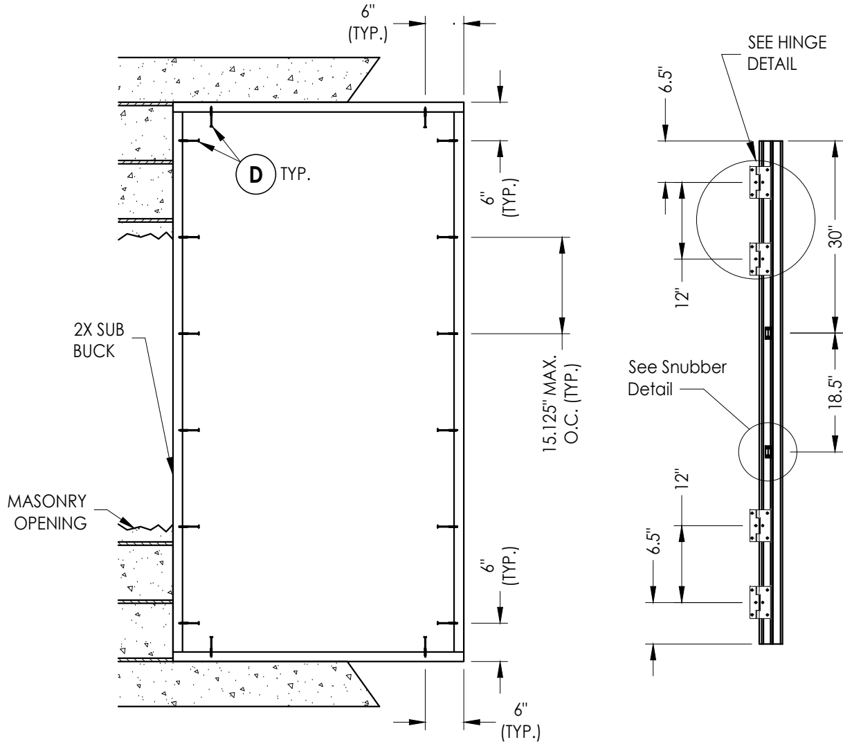
2X BUCK ANCHORING 42" X 84" Max Size
